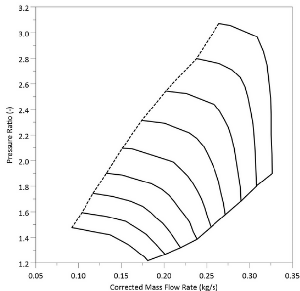
1D Analysis Compressor Map
